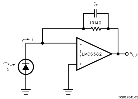
FIGURE 17. Photodiode Amplifier
